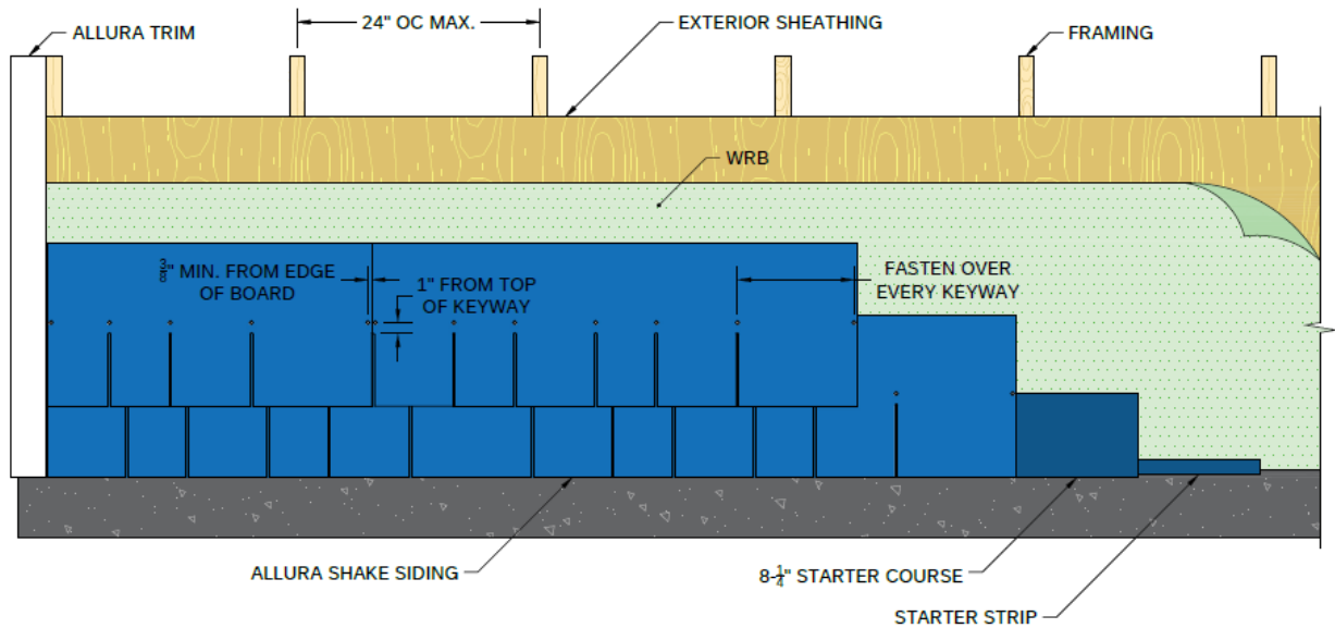
Figure 9 – Allura® and TerraPlank™ Shake Siding Blind Nail Fastening Details
