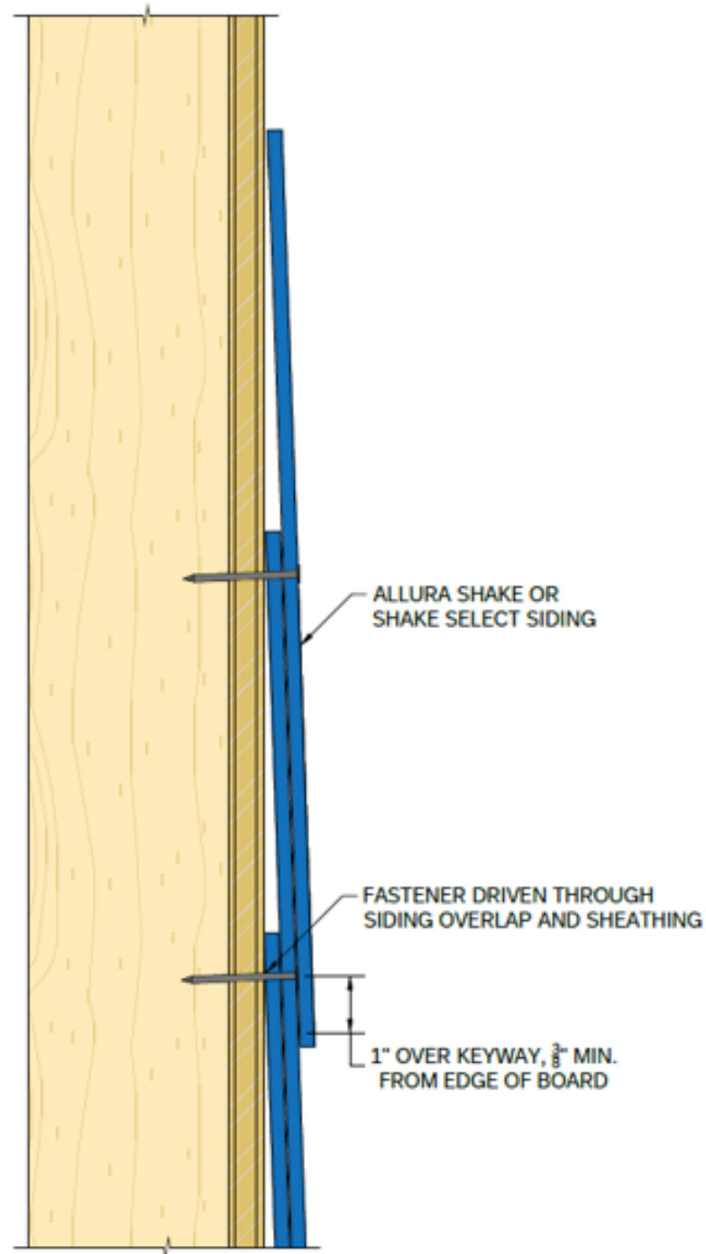
Figure 8 – Allura® and TerraPlank™ Shake and Allura® Shake Select General Installation
