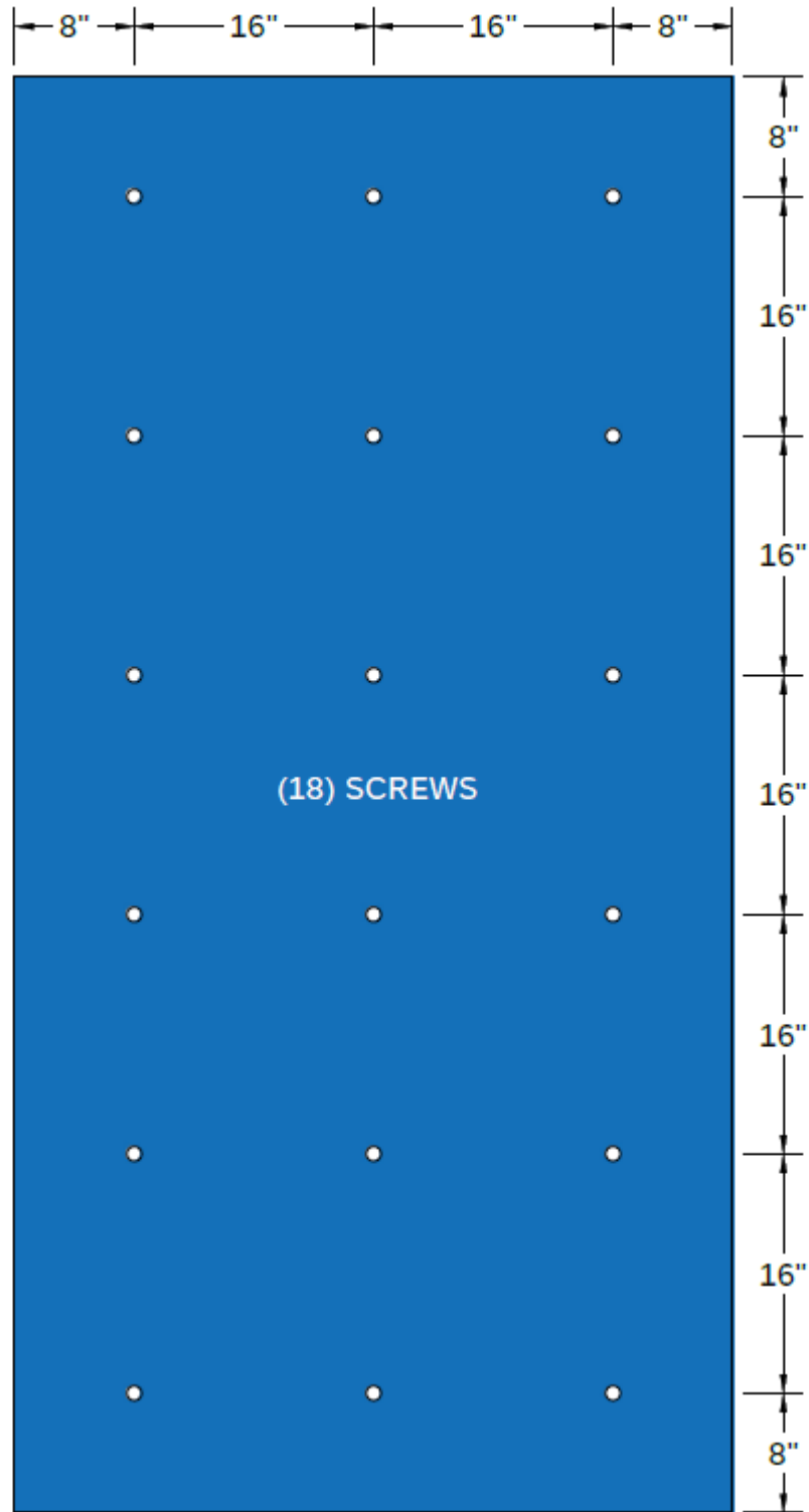
Figure 6 - Allura® and TerraPlank™ Panel Commercial Pattern “B”
