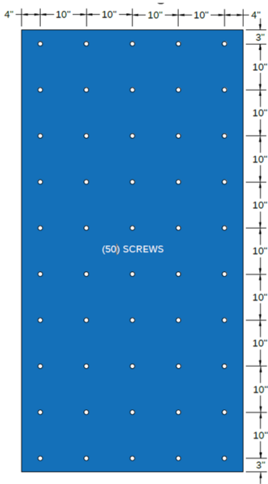
Figure 7: Allura® and TerraPlank™ Panel 3-4-10 Pattern
