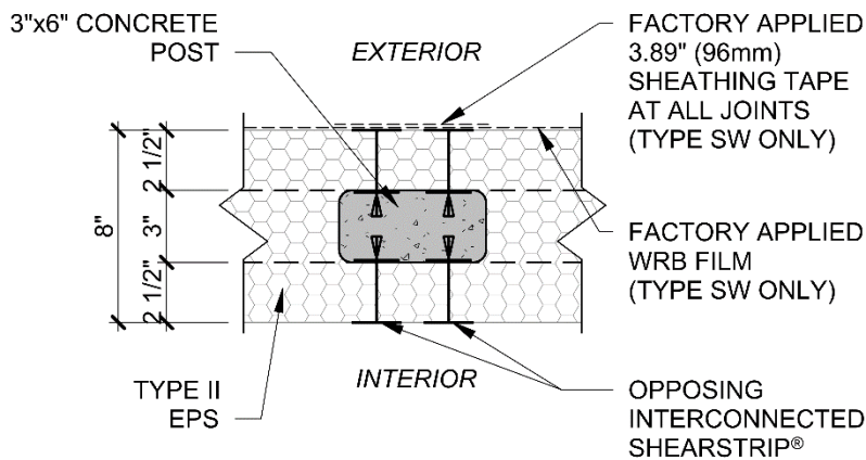
Figure 8. HercuWall® and HercuWall® HD Series 8 Type S, SW, and A Double Post Details
