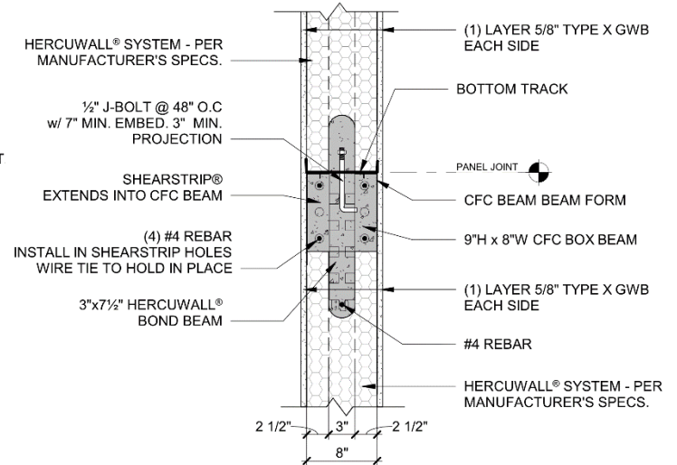
Figure 29– 1-hr Load-Bearing Unbraced CFC Box Beam Wall for Townhouses and Two- Family Dwellings. IRC Section 302.2 compliant where tight to exterior sheathing and Section 302.3 compliant where tight to exterior wall, where assembly extends to roof sheathing.
