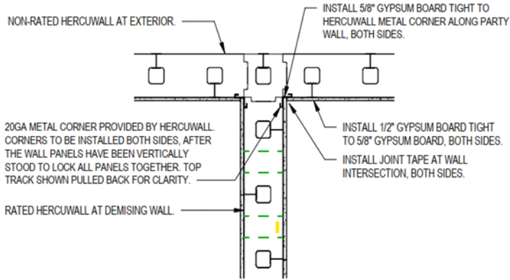
Figure 28 – 1-hr Load-bearing Common Wall for Two-Family Dwellings. IRC Section 302.3 compliant where assembly extends to roof sheathing.
