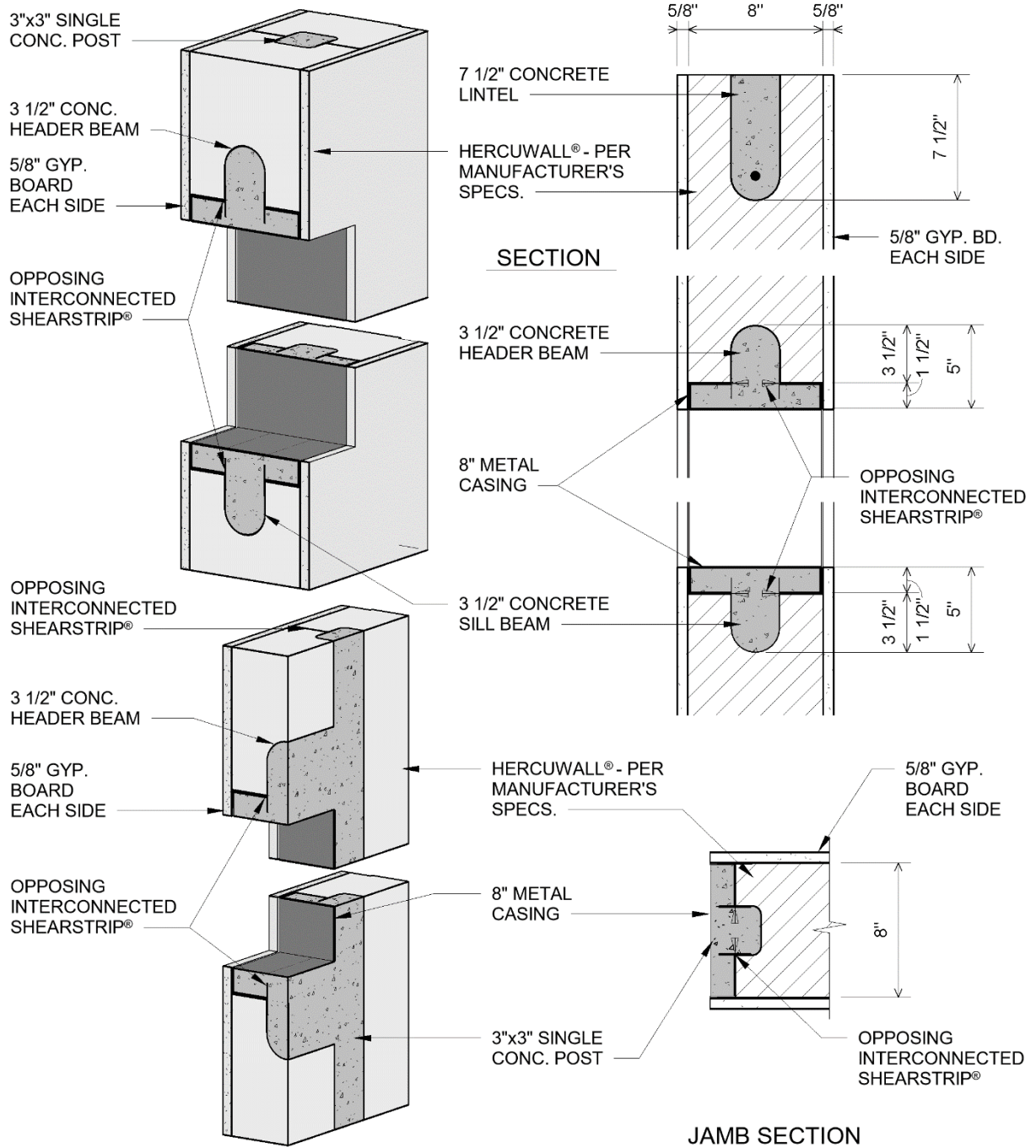
Figure 38. HercuWall® and HercuWall® HD Openings (Window and Door) Opening Design for Types I-IV Construction.
