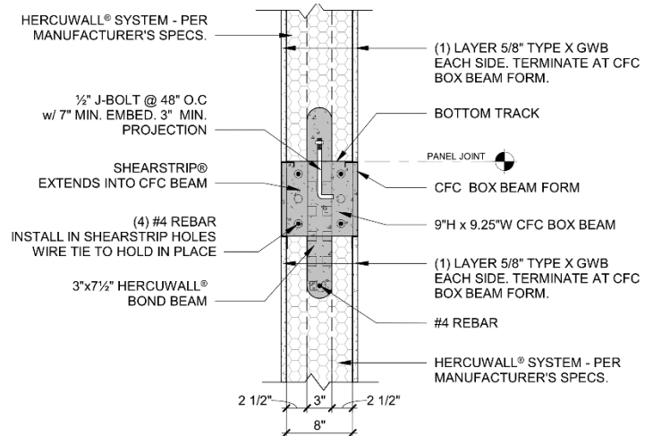
Figure 25– 1-hr Load-Bearing Unbraced CFC Box Beam Wall for Townhouses and Two-Family Dwellings. IRC Section 302.2 compliant where tight to exterior sheathing and Section 302.3 compliant where tight to exterior wall, where assembly extends to roof sheathing.
