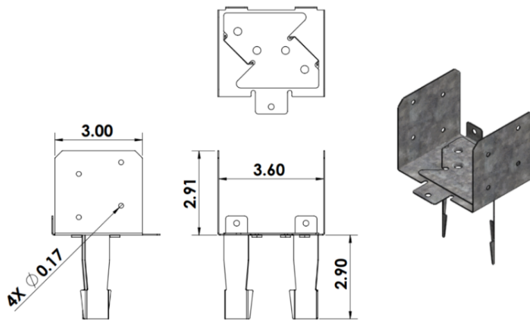
Figure 14 - HercuWall® and HercuWall® HD Truss Saddle Bracket
