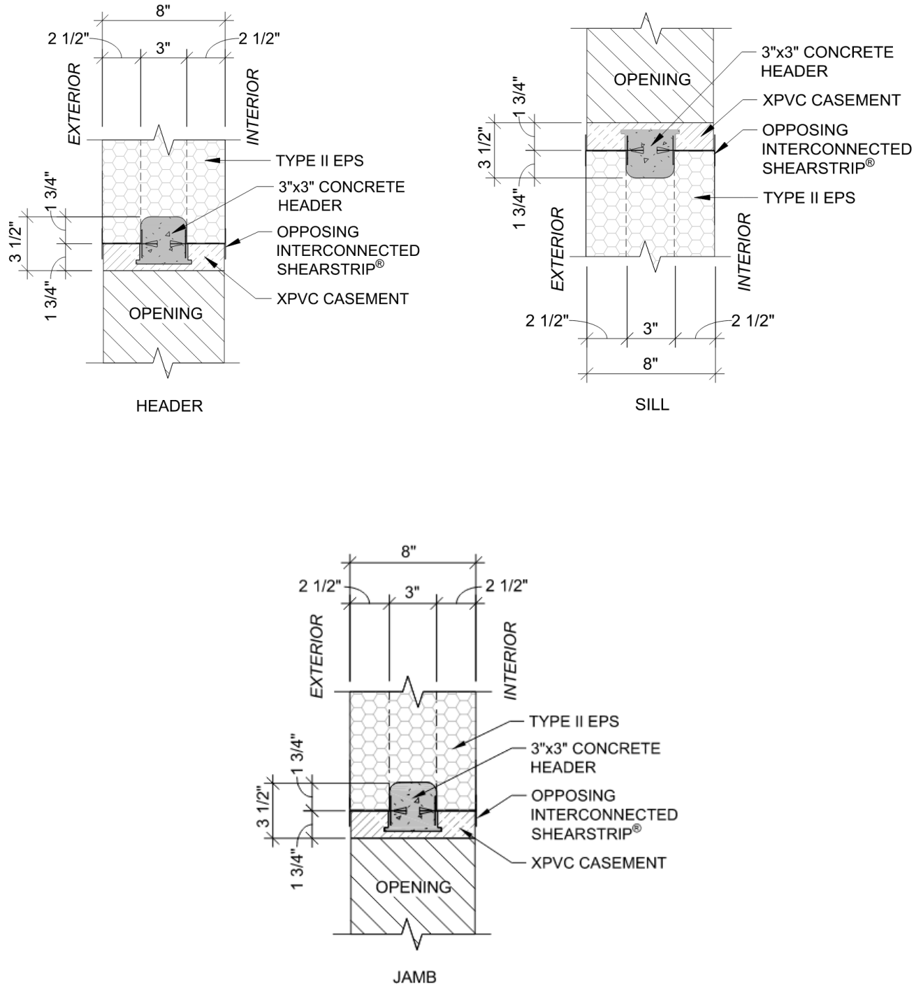
Figure 11 – HercuWall® and HercuWall® HD Series 8 Header, Sill and Jamb Sections – Composite Casing
