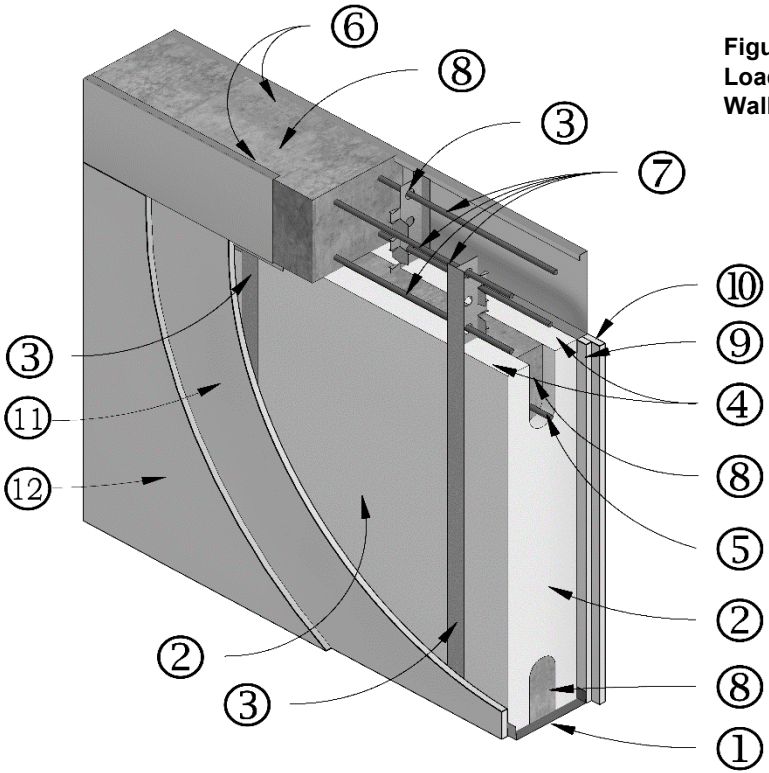
Figure 31b. HercuWall® and HercuWall® HD 2-Hour Load-Bearing Fire-Resistance Rated CFC Box Beam Wall Assembly Design.
