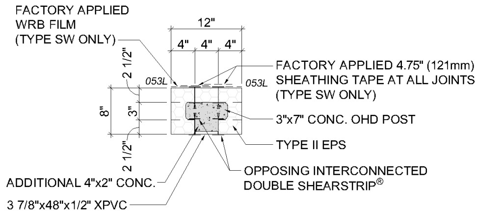
Figure 8. HercuWall® and HercuWall® HD Series 8 Type S, SW, and A Post Details
