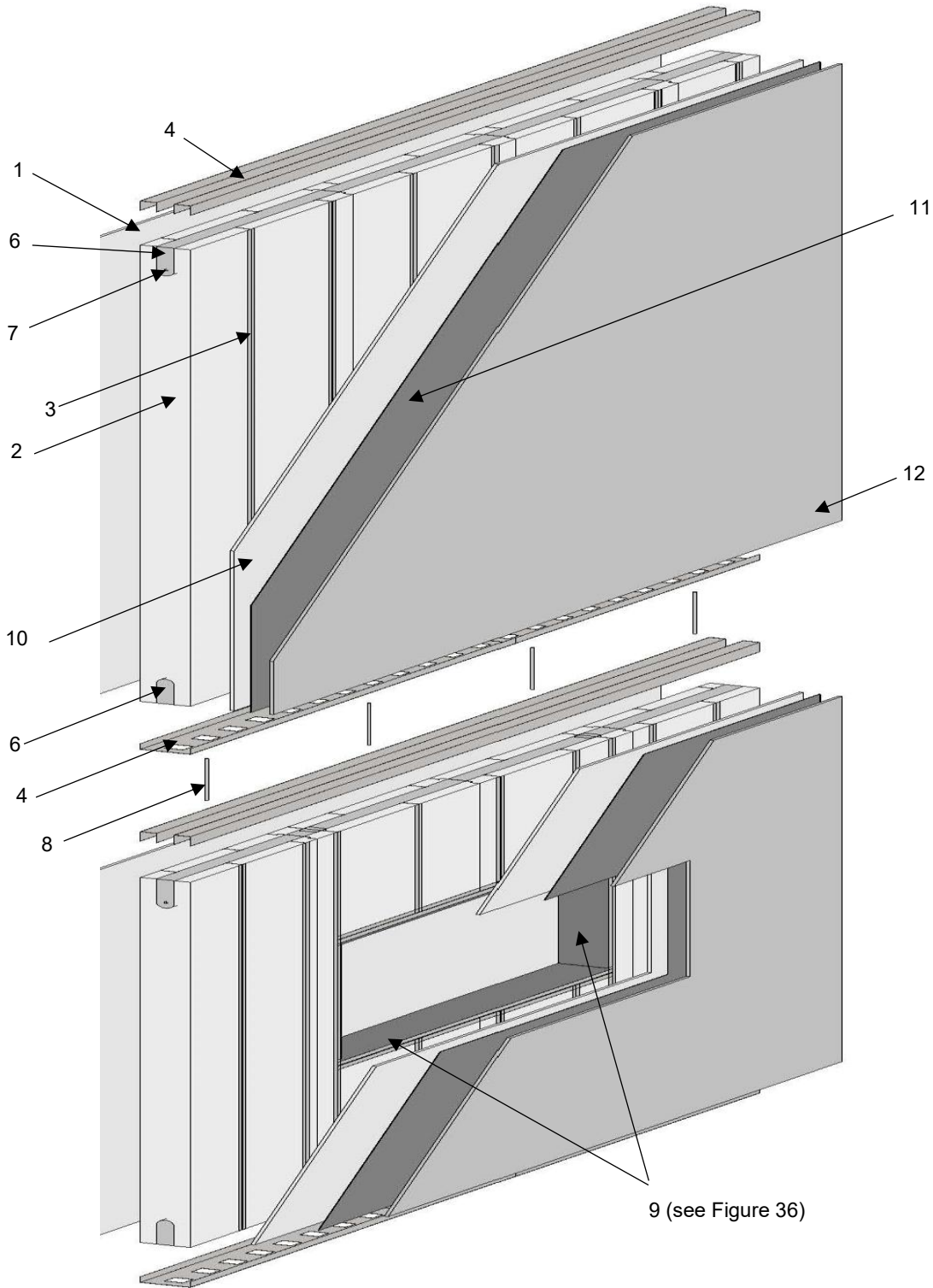
Figure 37. HercuWall® Types I-V Construction Design
