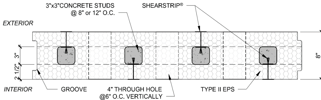
Figure 7. HerculWall® and HerculWall® HD Series 8 Type A Panel Details
