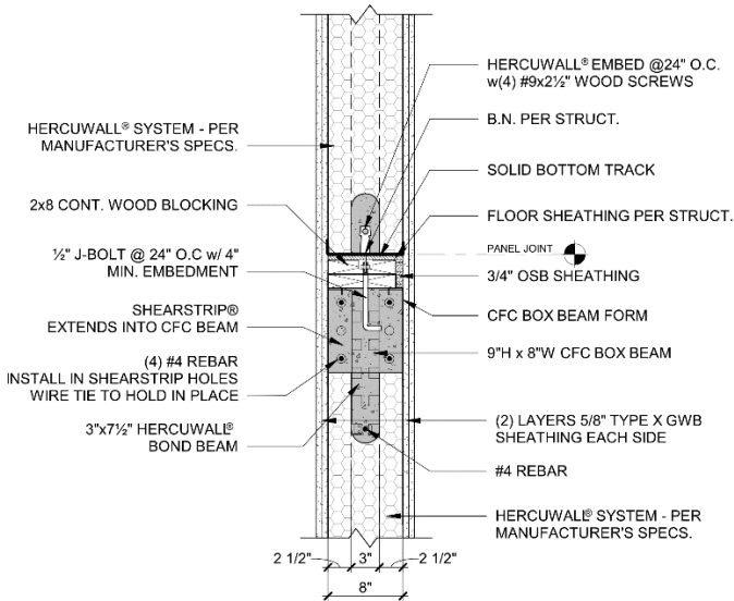
Figure 32 – 2-hr Load-Bearing Unbraced CFC Box Beam Wall
