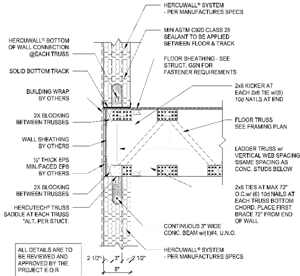
Figure 18 – Typical Truss Perpendicular to Wall (Section)
