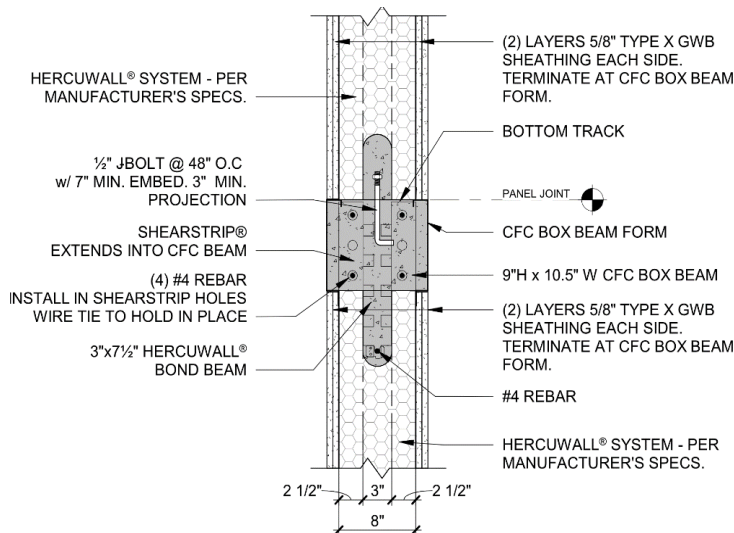
Figure 34 – 2-hr Load-Bearing Braced CFC Box Beam Wall approved for Fire Wall and Party Wall where Installed per IBC Section 706 (Type V construction). Approved for Townhouses where installed per IRC Section 302.2 and Two Family Dwellings where installed per IRC Section 302.3.
