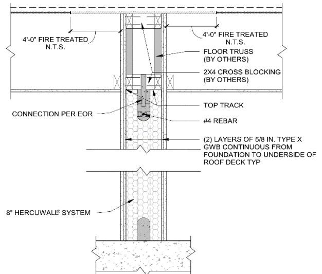
Figure 35 – 2-hr Load-bearing Attic Transition for Townhouses and Two Family Dwellings IRC Section 302.2 compliant where tight to exterior sheathing and Section 302.3 compliant where tight to exterior wall
