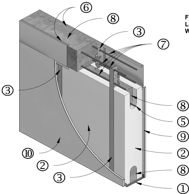
Figure 23b. HercuWall® and HercuWall® HD 1-Hour Load-Bearing Fire-Resistance Rated CFC Box Beam Wall Assembly Design.
