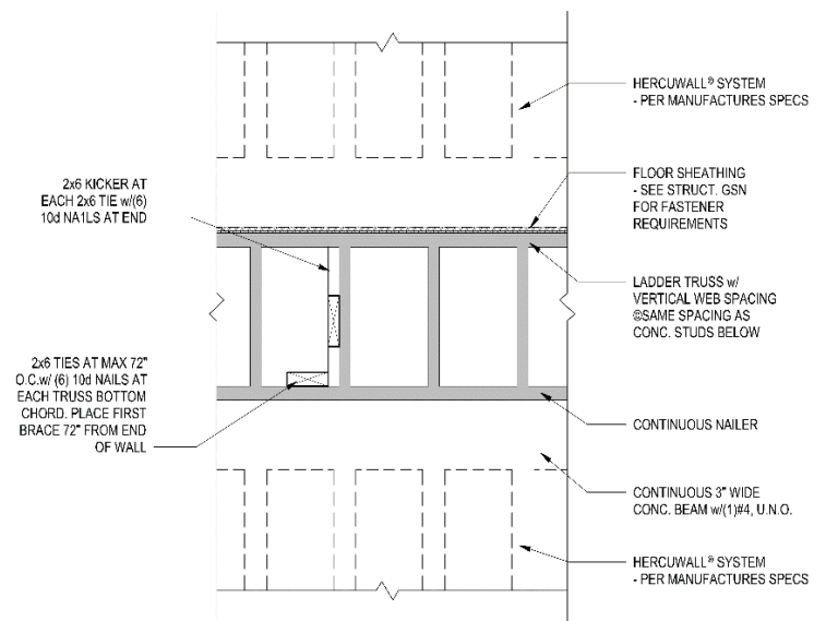
Figure 21 – Typical Truss Parallel to Wall (Elevation)
