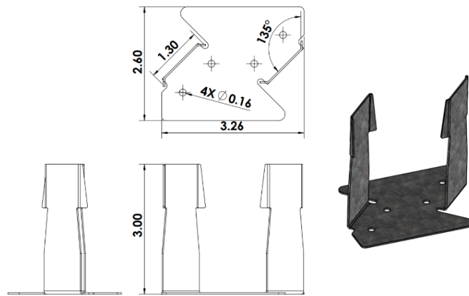
Figure 13 - HercuWall® and HercuWall® HD Embed
