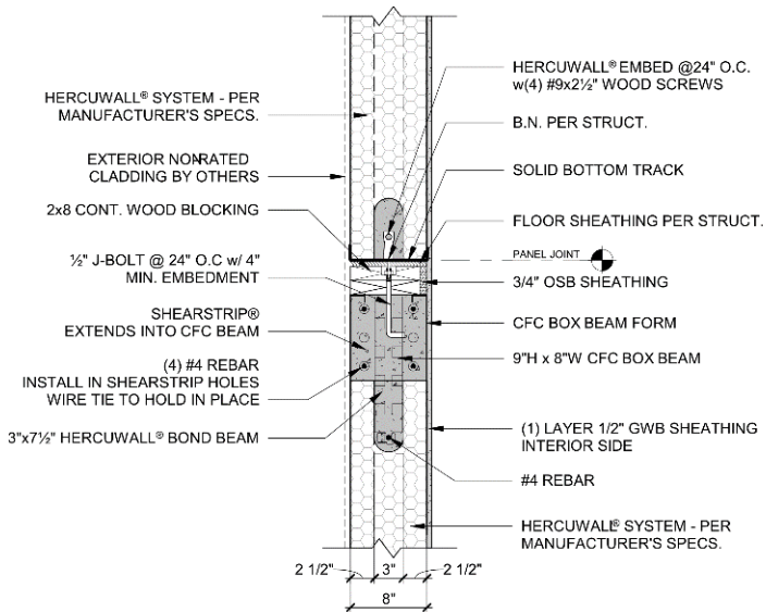
Figure 16 – Typical CFC Box Beam Wall Construction with Lumber Embed
