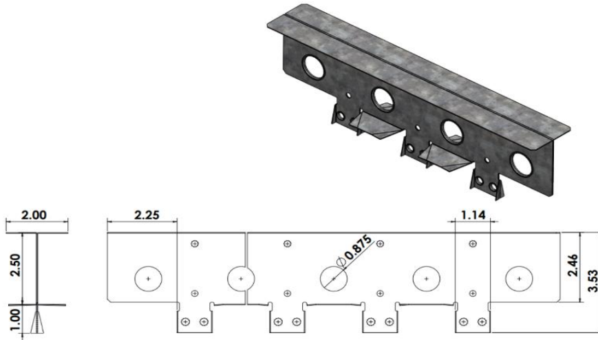
Figure 12 - HercuWall® and HercuWall® HD ShearStrip
