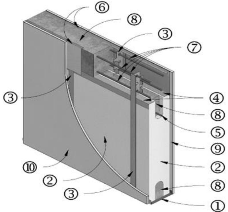
Figure 23a. HercuWall® and HercuWall® HD 1-Hour Load-Bearing Fire-Resistance Rated CFC Box Beam Wall Assembly Design.
