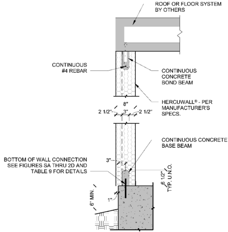
Figure 15 – Typical Wall Section
