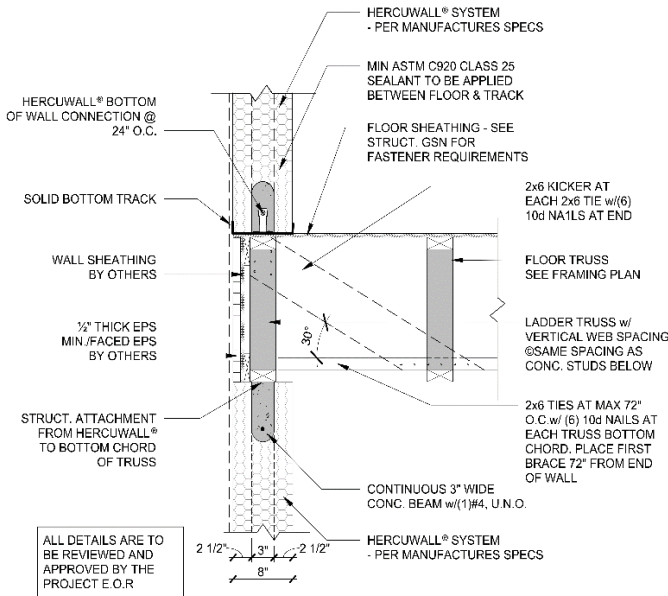
Figure 20 – Typical Truss Parallel to Wall (Section)
