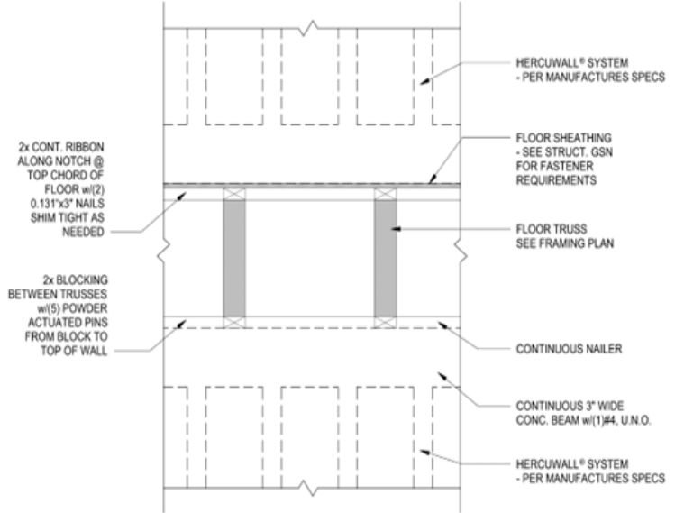
Figure 19 – Typical Truss Perpendicular to Wall (Elevation)
