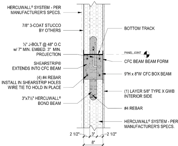
Figure 26 – 1-hr Load-Bearing Unbraced CFC Box Beam Wall
