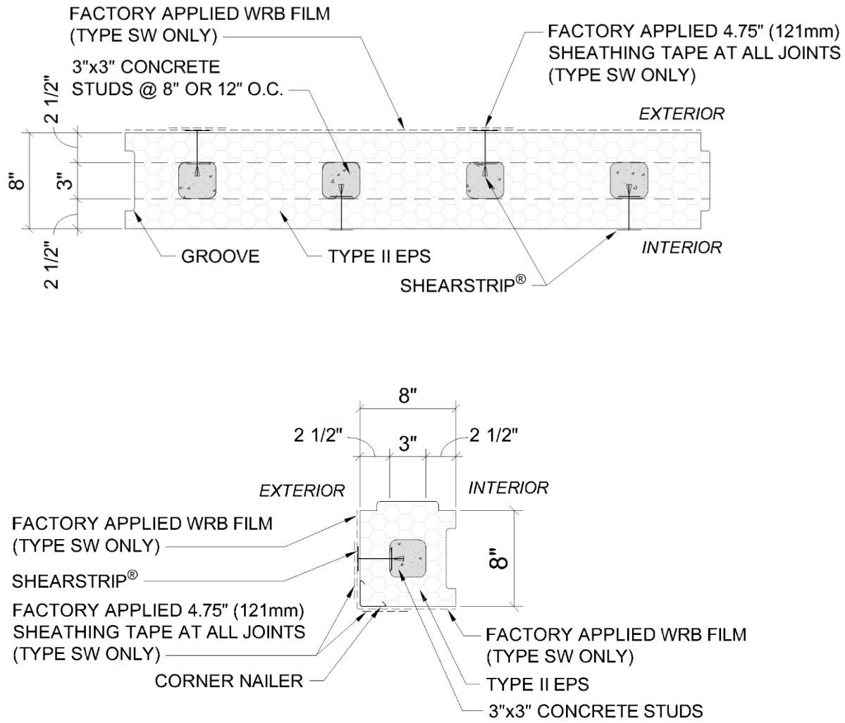
Figure 5. HercuWall® and HercuWall® HD Series 8 Type S and SW Panel and Corner Details
