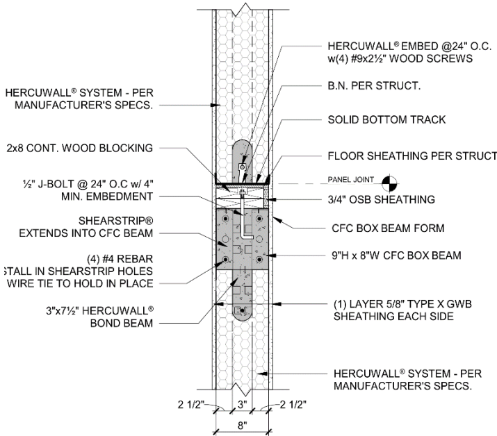
Figure 24 – 1-hr Load-Bearing Unbraced CFC Box Beam Wall
