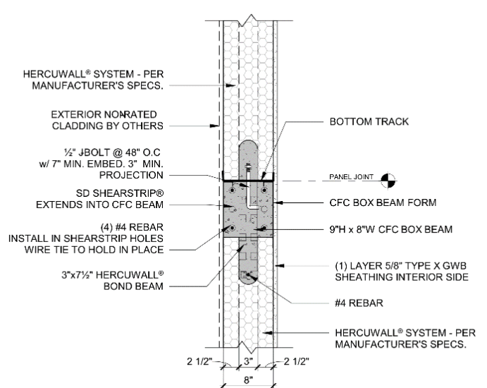
Figure 17– Typical CFC Box Beam Wall Construction Concrete Option
