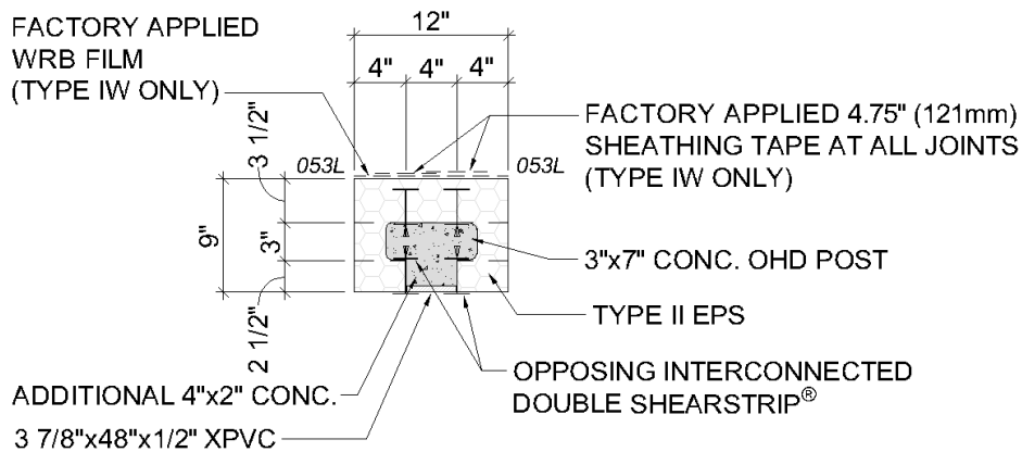
Figure 9. HercuWall® and HercuWall® HD Series 8 Type I and IW Post Details
