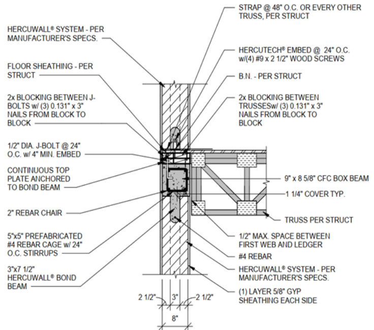
1-hr Load-Bearing Braced (1 Side) CFC Box Beam Wall 1
