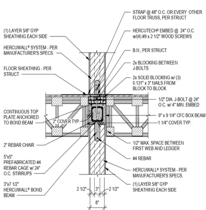
1-hr Load-Bearing Braced (2 Sides) CFC Box Beam Wall 1
