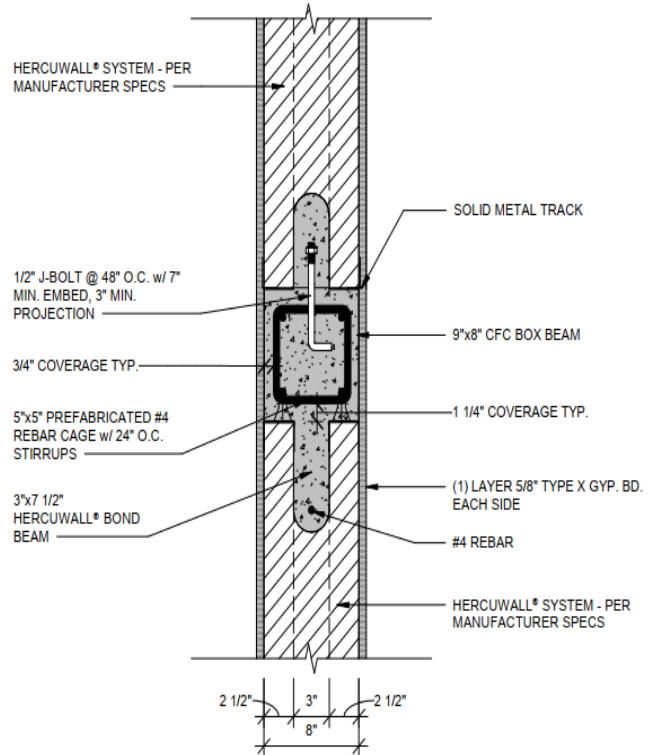
1-hr Load-Bearing Unbraced CFC Box Beam Wall
