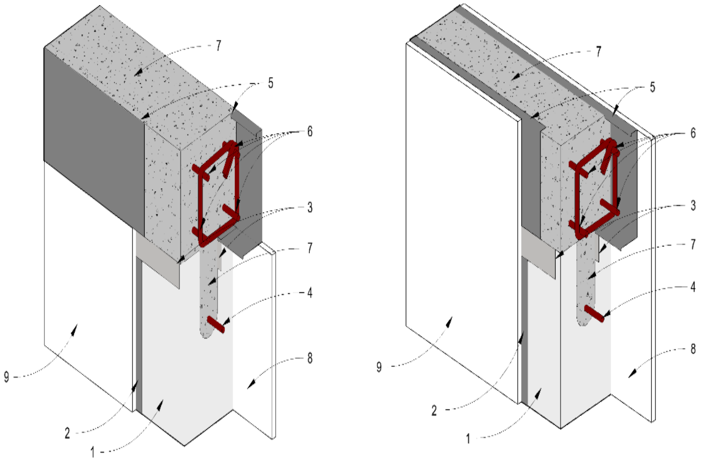
CFC Box Beam 1 Hour Load-Bearing Fire-Resistance Rating Application Details
