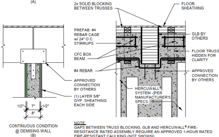
1-hr Beam Penetration of Load-Bearing CFC Box Beam Wall
