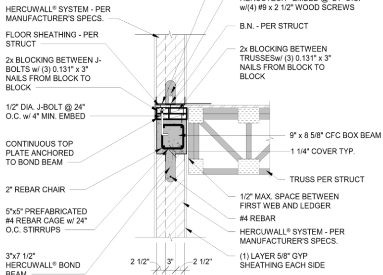
1-hr Load-Bearing Braced (1 Side) CFC Box Beam Wall
