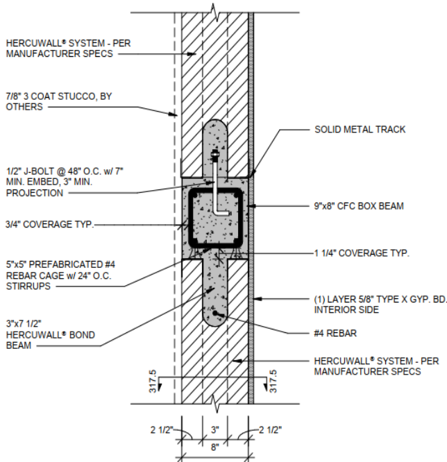
1-hr Load-Bearing Unbraced CFC Box Beam Wall
