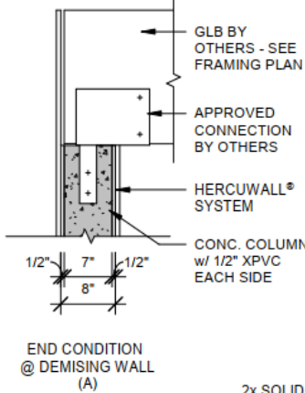
1-hr Load-Bearing Braced (2 Sides) CFC Box Beam Wall
