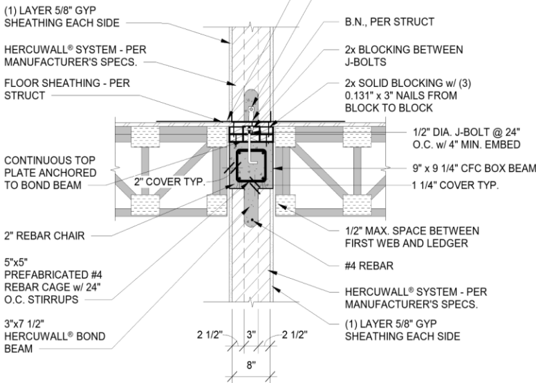
1-hr Load-Bearing Braced (2 Sides) CFC Box Beam Wall
