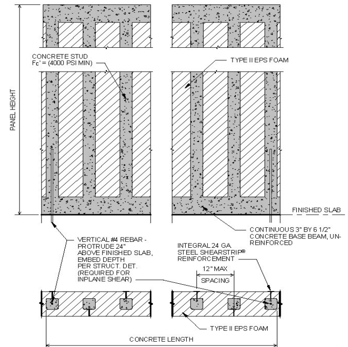
Figure 16– Typical Unreinforced Wall Section and Elevation
