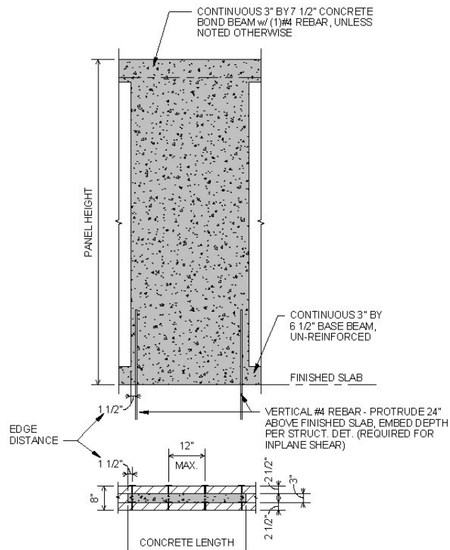
Figure 18– Typical Unreinforced Solid Shear Wall Section and Elevation
