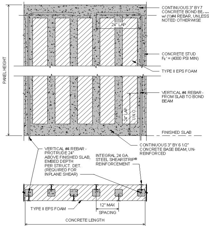
Figure 17– Typical Reinforced Wall Section and Elevation
