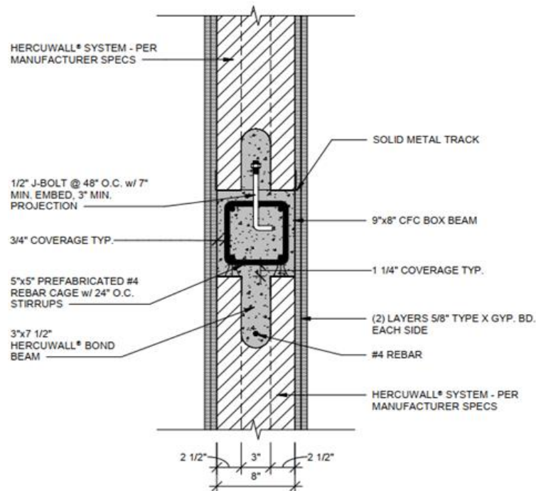
Figure 35 – 2-hr Load-Bearing Unbraced CFC Box Beam Wall
