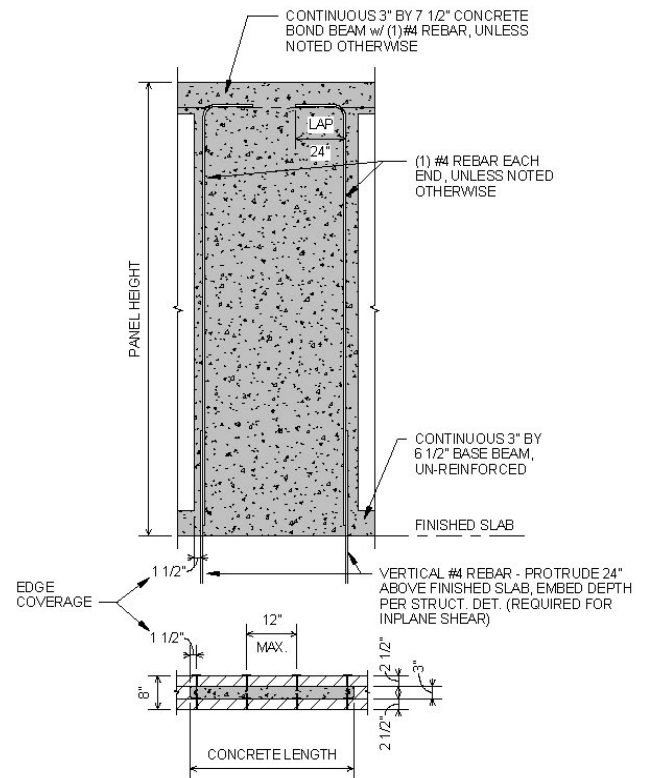
Figure 19– Typical Reinforced Solid Shear Wall Section and Elevation
