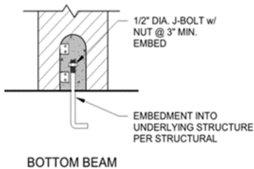
Figure 2C – J-Bolt
