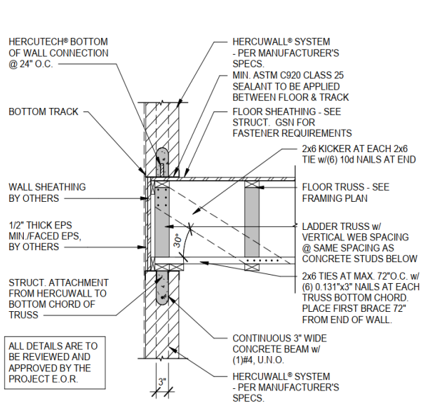
Figure 25 – HercuWall® Truss Parallel to Wall (Section)
