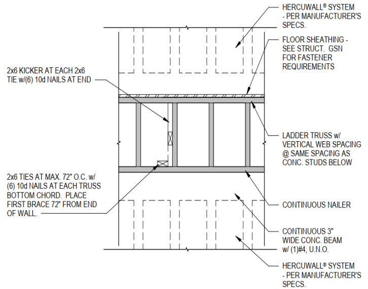
Figure 26 – HercuWall® Truss Parallel to Wall (Elevation)
