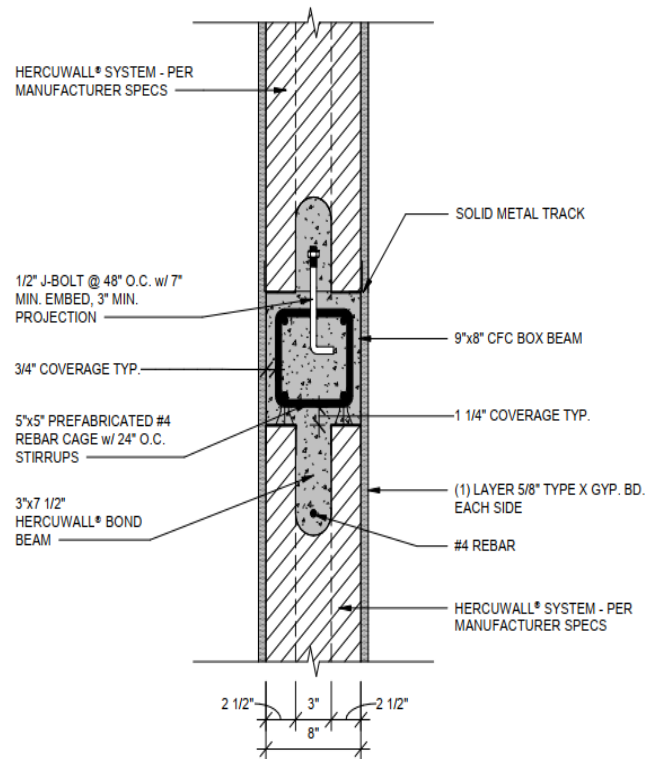
Figure 30– 1-hr Load-Bearing Unbraced CFC Box Beam Wall
