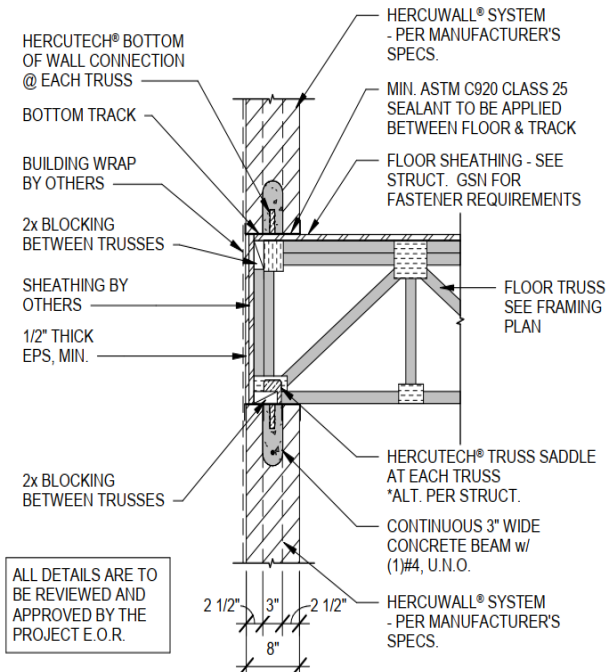
Figure 23 – HercuWall® Truss Perpendicular to Wall (Section)
