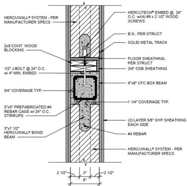
Figure 34 – 2-hr Load-Bearing Unbraced CFC Box Beam Wall
