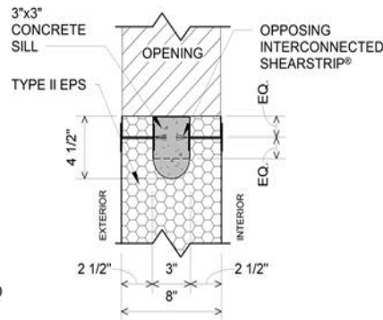
Figure 11B - Sill
