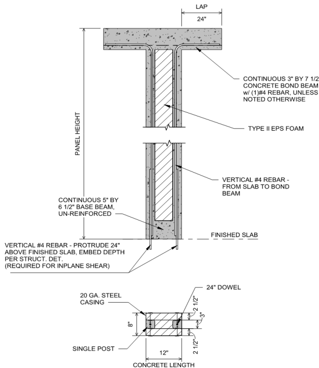
Figure 20– Typical Door / Window Between Panel Section and Elevation
