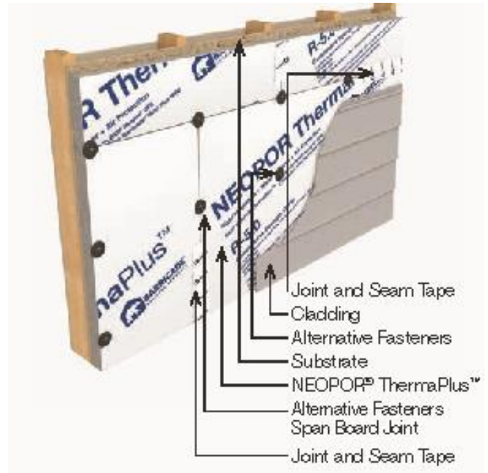
Figure 2. Alternate NEOPOR ThermaPlus™ Installation with Fastener Washer Spanning Joint.
