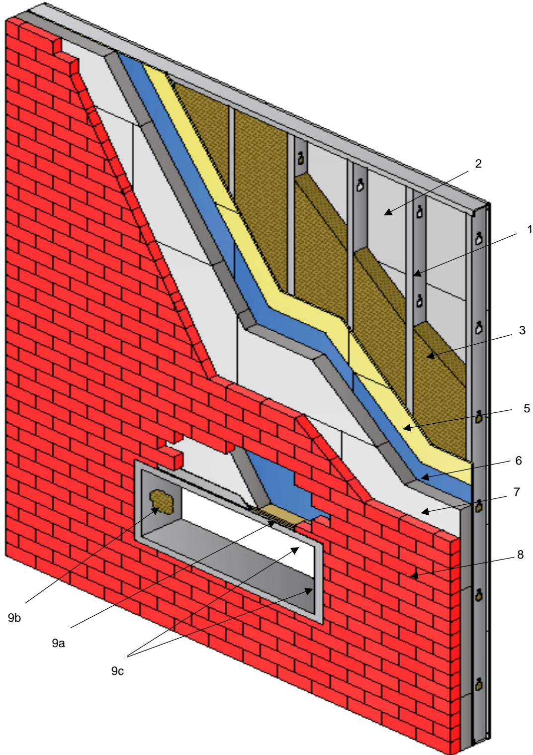
Figure 4. NEOPOR ThermaPlus™ Types I-IV Construction (NFPA 285) Approved Assemblies
