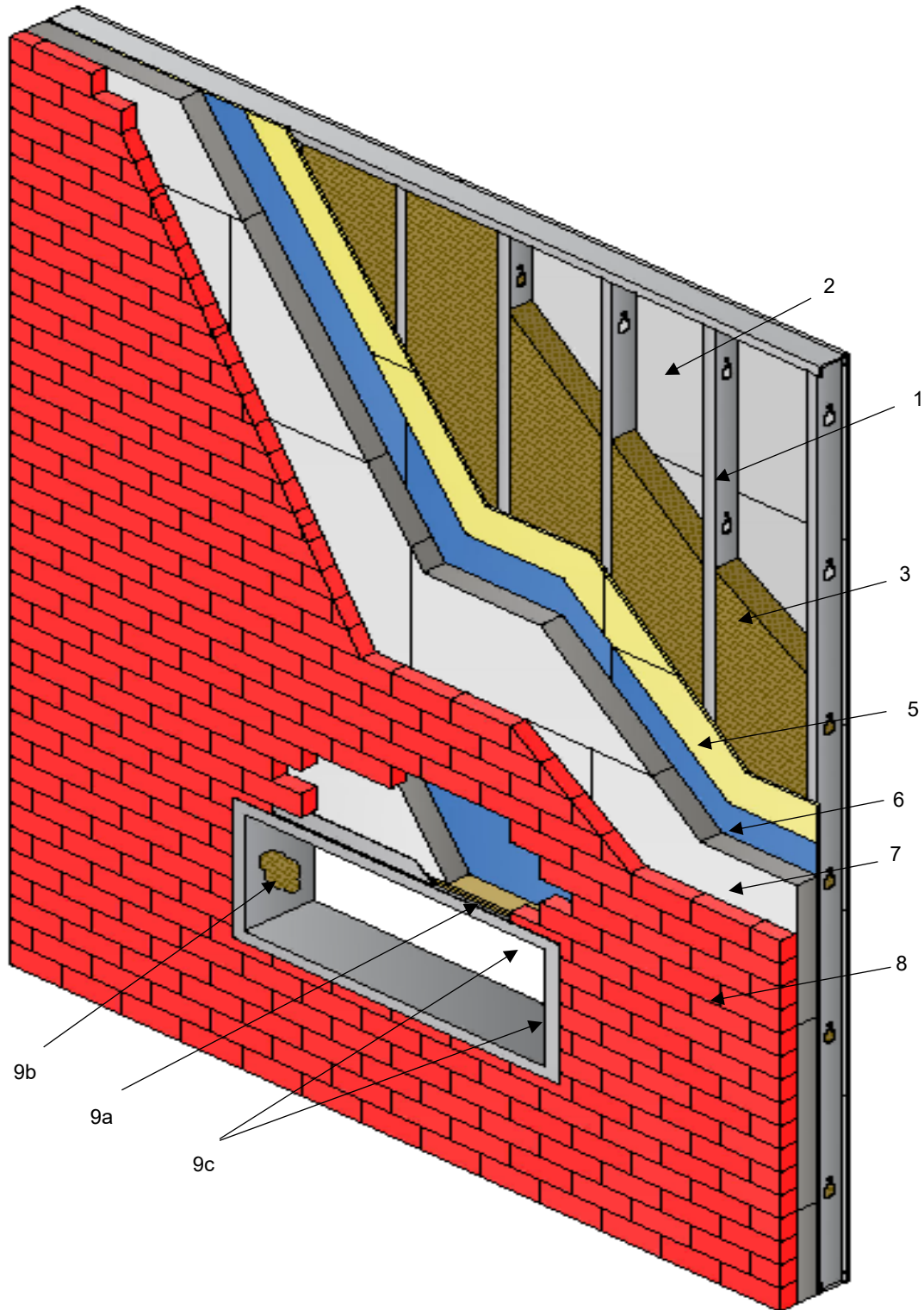
Figure 5. IntegraShield™ Types I-IV Construction (NFPA 285) Approved Assemblies
