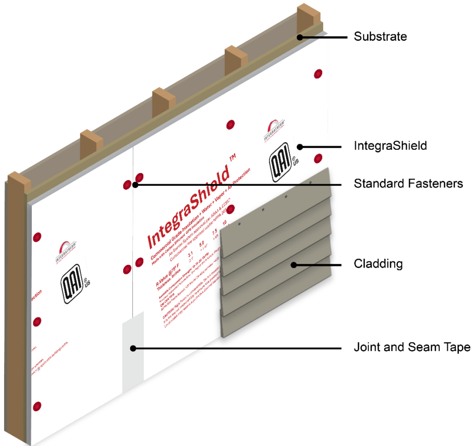
Figure 3. Standard IntegraShield™ Water-Resistive Barrier Insulation 1,2,3
