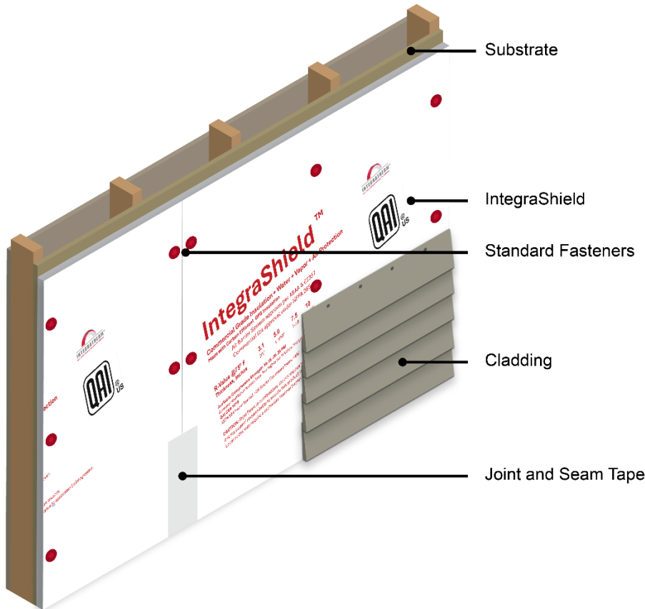
Figure 4. Standard IntegraShield™ Installation with Fasteners on Each Joint Edge.
