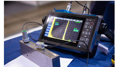
Ultrasonic Testing
